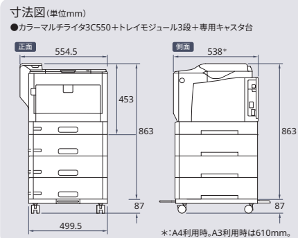
Color MultiWriter 3C550
