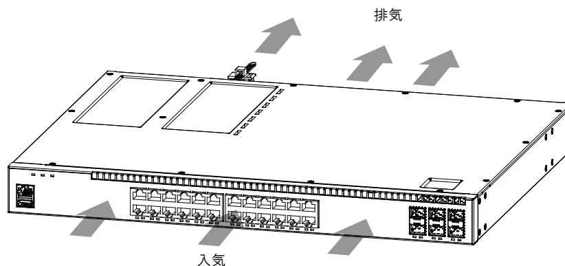
図2-7 IP8800/S2340-48T4X , IP8800/S2340-24P4X , IP8800/S2340-48P4X , IP8800/S2340-16P8MP2X のエアフロー
