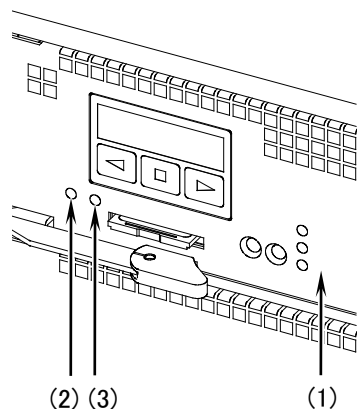
図4-62 LED の確認
