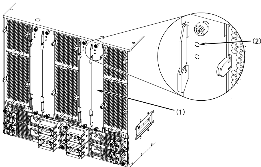
図5-35 STATUS LED の確認
