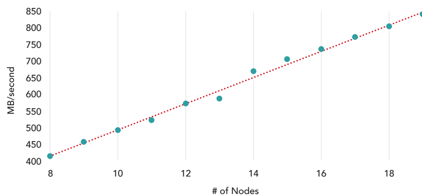
Figure 3: k-means median throughput.
